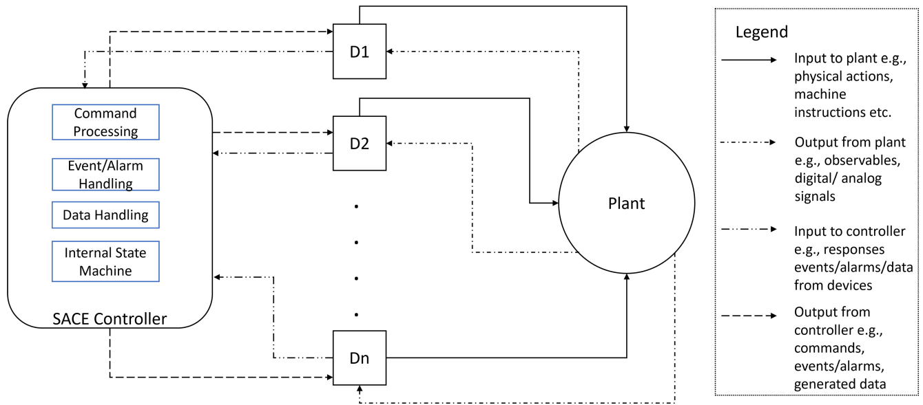
Fig. 5. SACE architecture.
